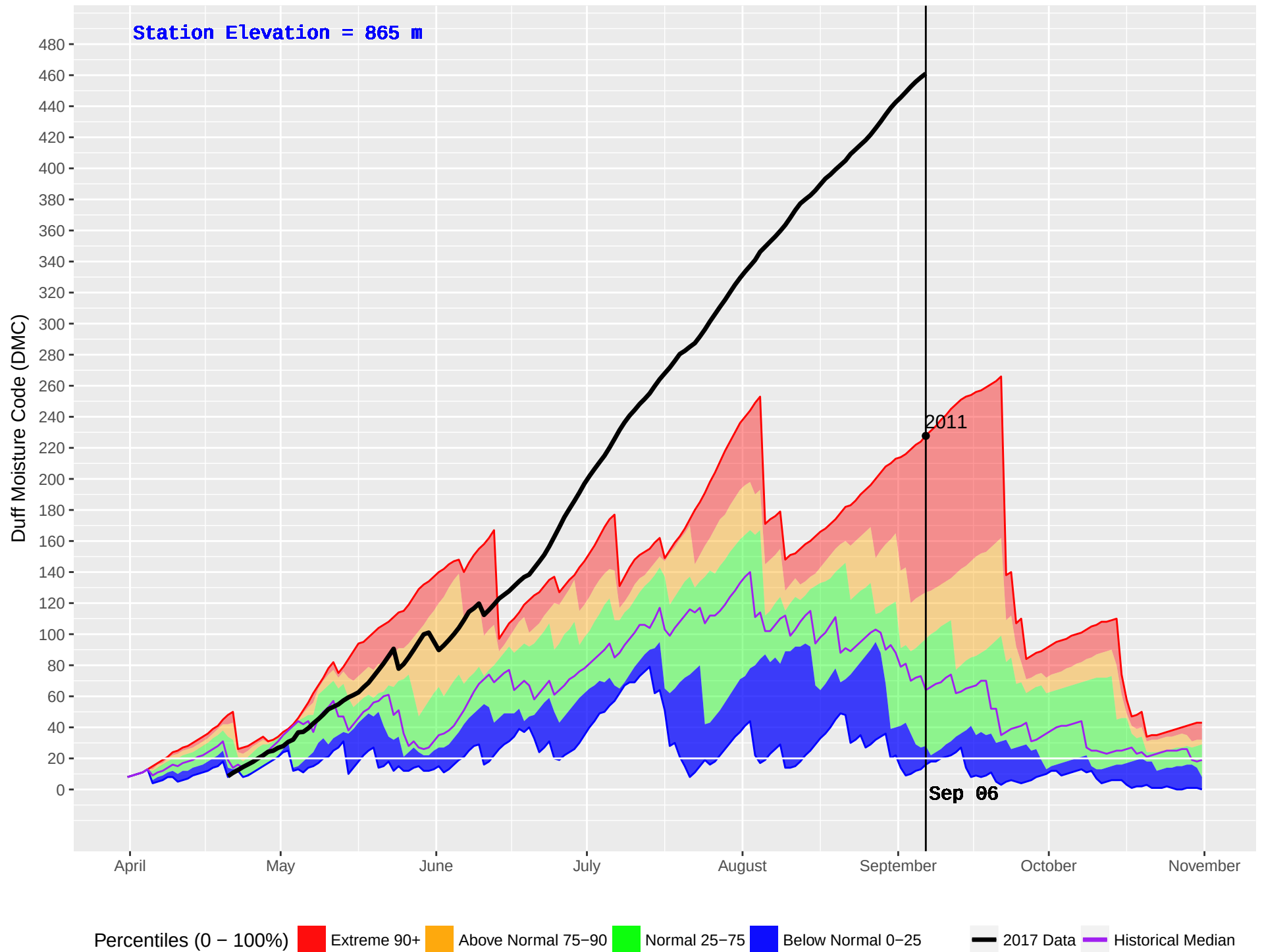
FIVE MILE (1029) : Historical (2008–2016) and Current (2017) Noon Duff Moisture Code (DMC)
