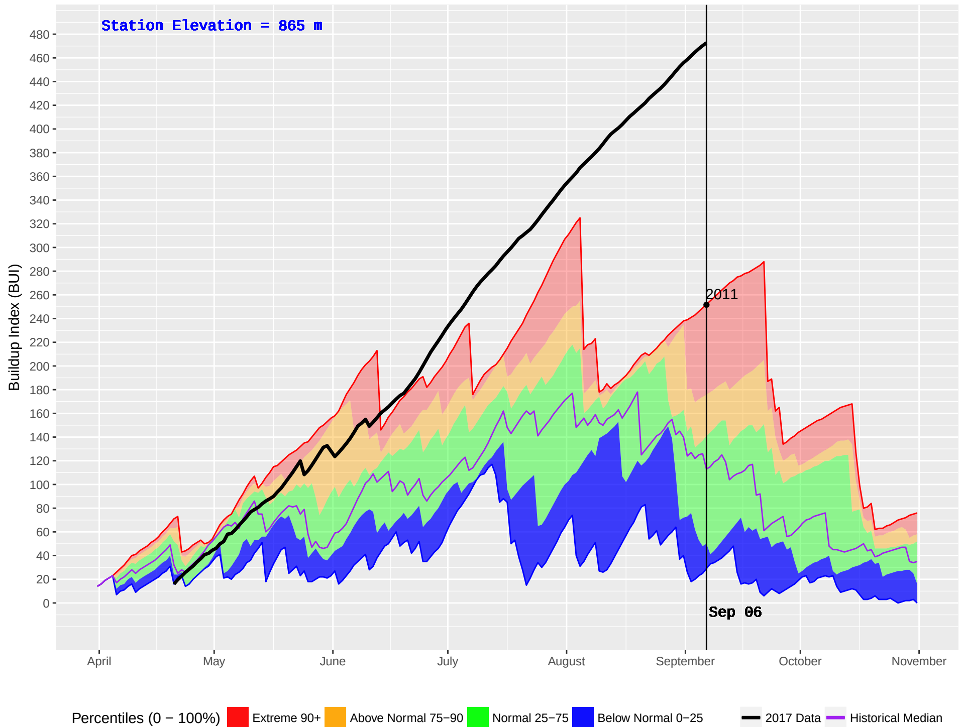
FIVE MILE (1029) : Historical (2008–2016) and Current (2017) Noon Buildup Index (BUI)
