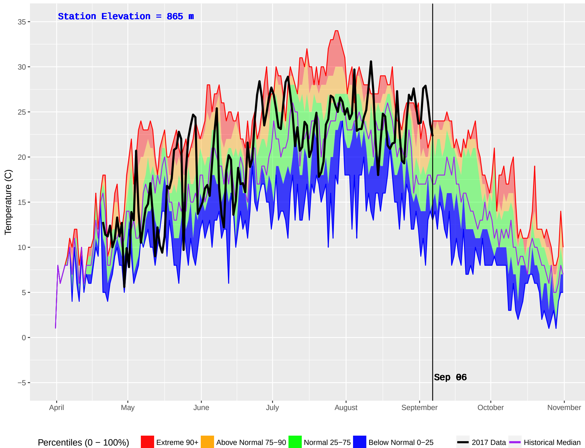
FIVE MILE (1029) : Historical (2008–2016) and Current (2017) Noon Temperature
