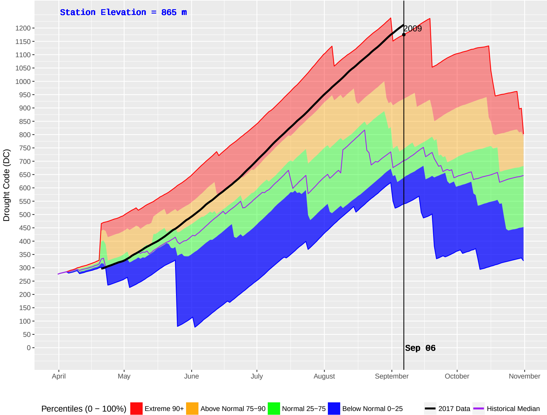
FIVE MILE (1029) : Historical (2008–2016) and Current (2017) Noon Drought Code (DC)
