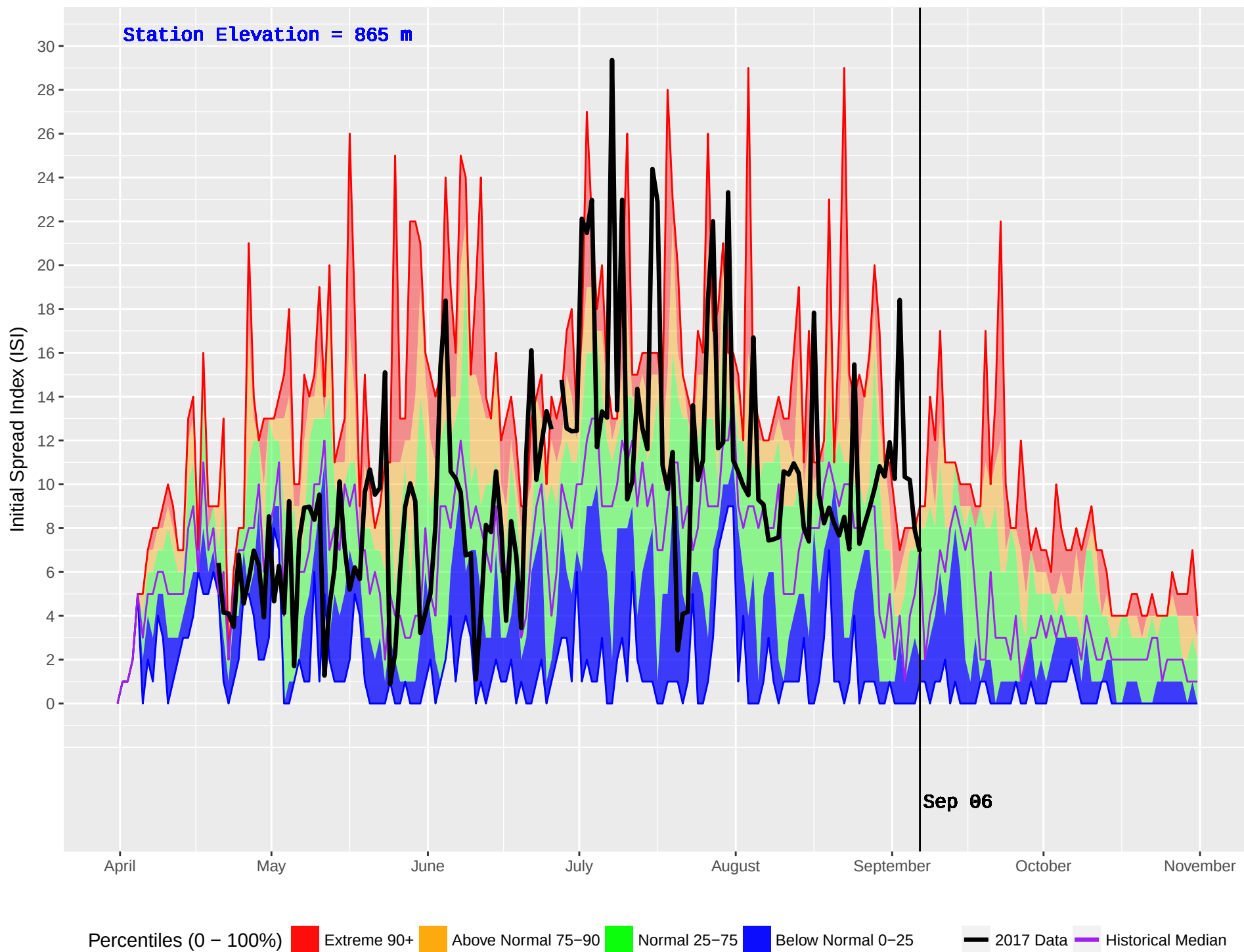
FIVE MILE (1029) : Historical (2008–2016) and Current (2017) Noon Initial Spread Index (ISI)
