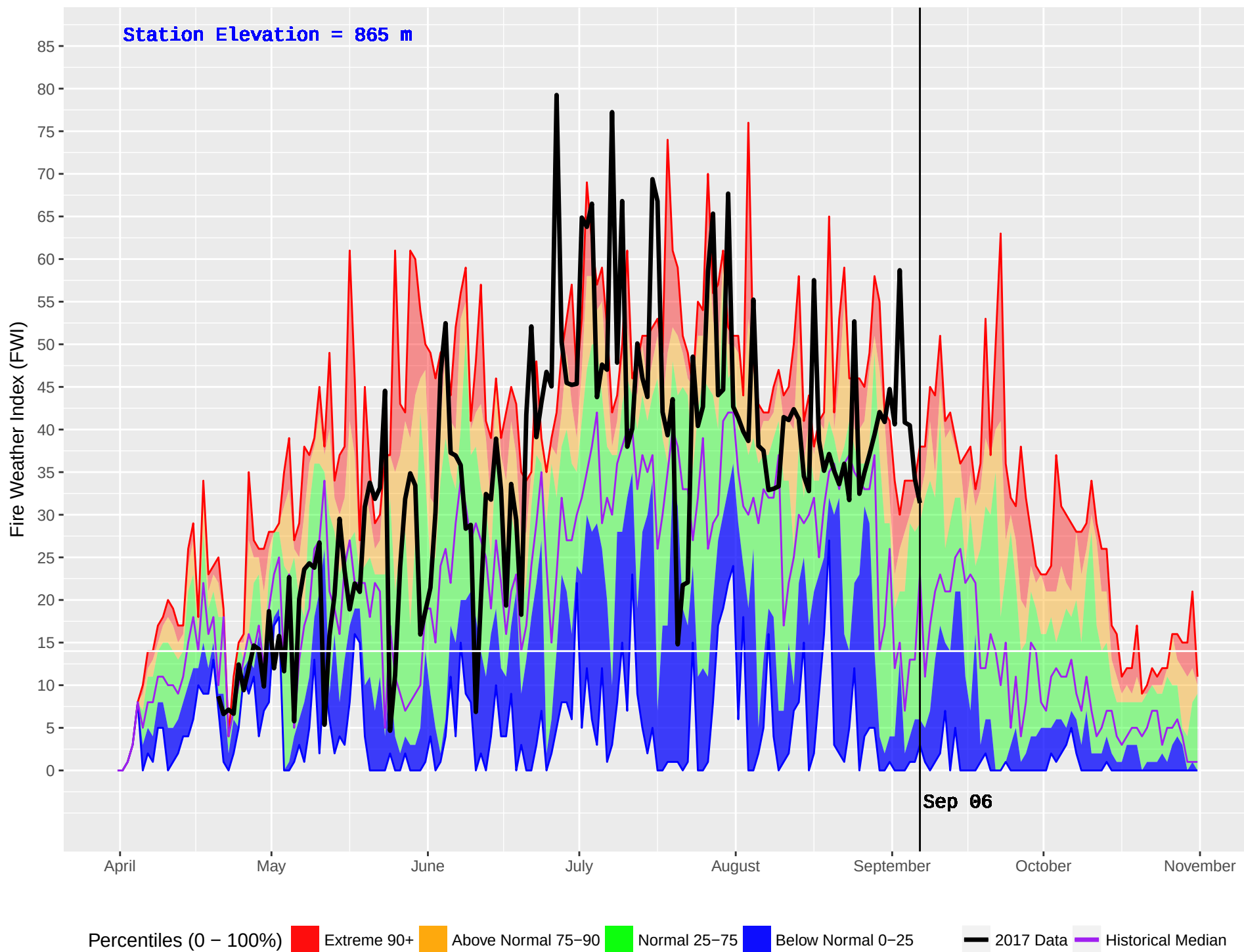
FIVE MILE (1029) : Historical (2008–2016) and Current (2017) Noon Fire Weather Index (FWI)
